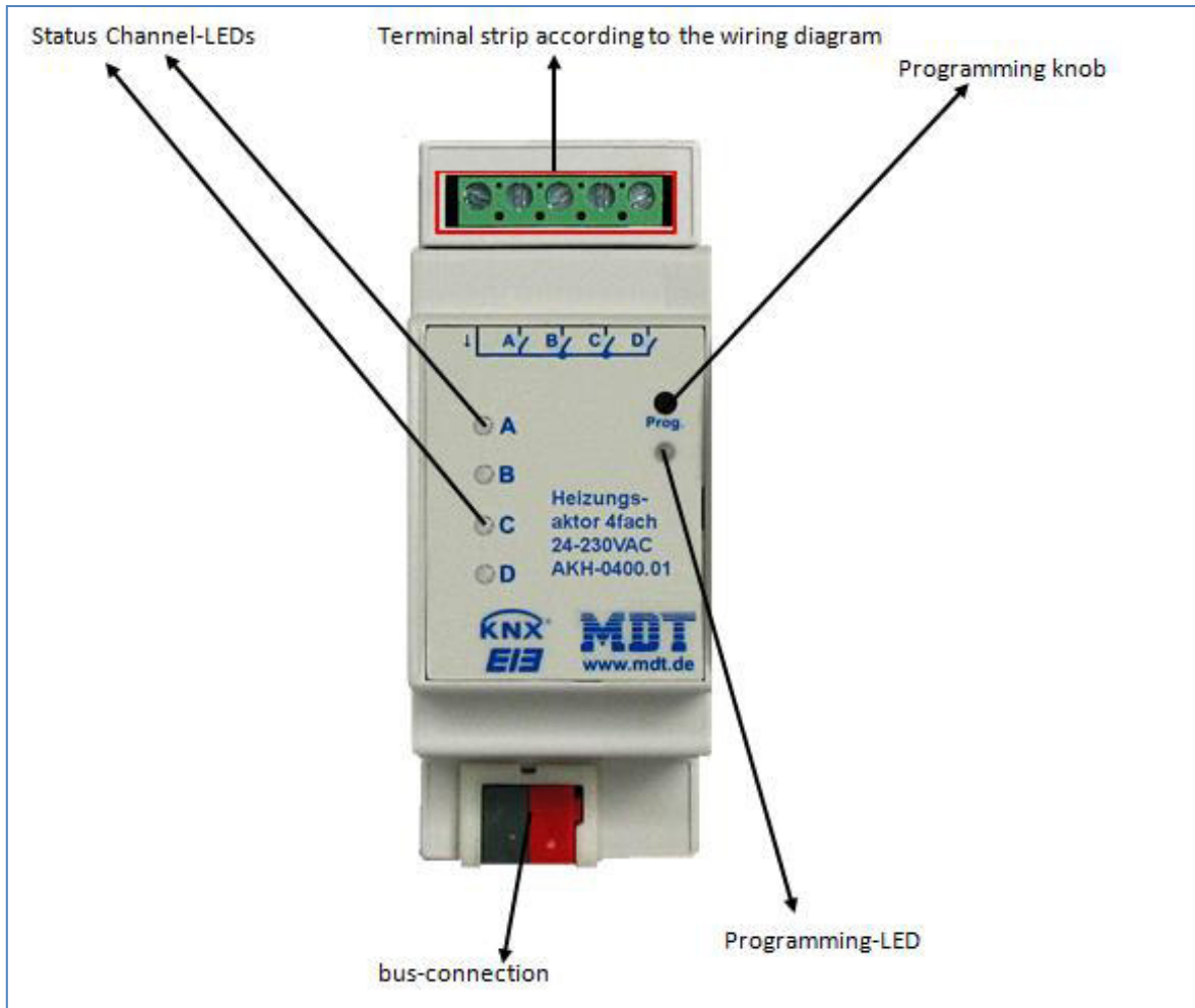
Figure 3: Overview hardware module
